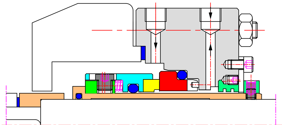
90 SERIES MULTI SPRINGS MECHANICAL SEAL TYPE 9201 CARTRIDGE ARRANGEMENT WITH DIFFERENT API PLAN 11& 62
